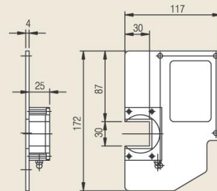
Wiper & Lubrication Unit
